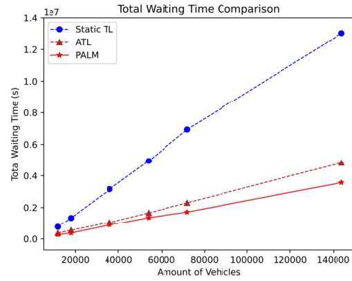
Fig. 6. Comparison of the total waiting time.
