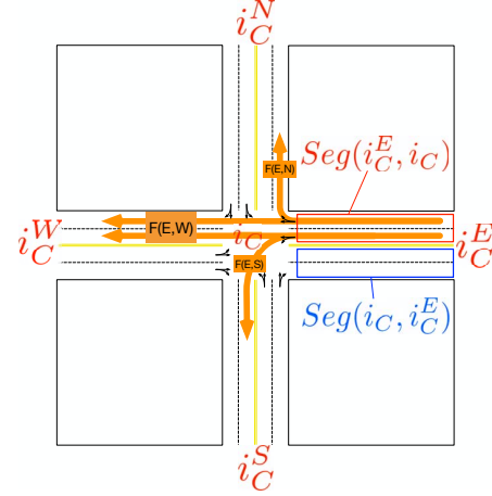
Fig. 1. Intersection, Segment and Traffic Flow.
